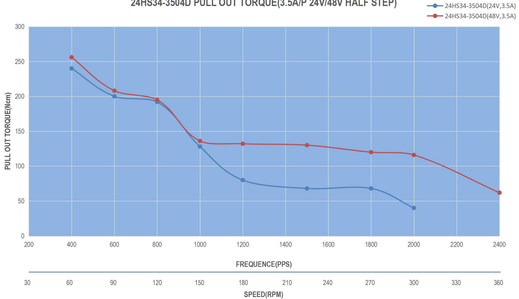
24HS34-3504D PULL OUT TORQUE(3.5A/P 24V/48V HALF STEP)
