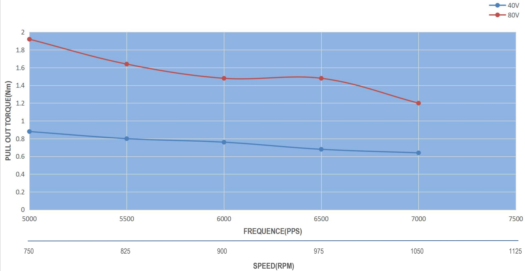
34HS38-3008S PULL OUT TORQUE(5.1A/P 40V/80V HALF STEP)
