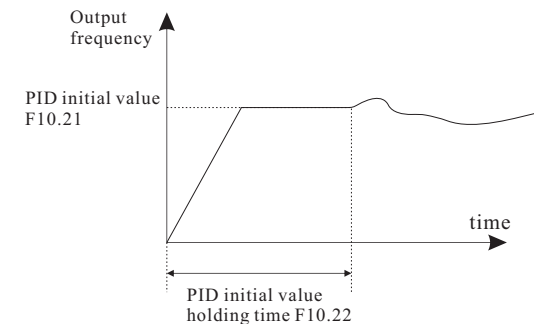
Figure 6-31 PID initial value function
