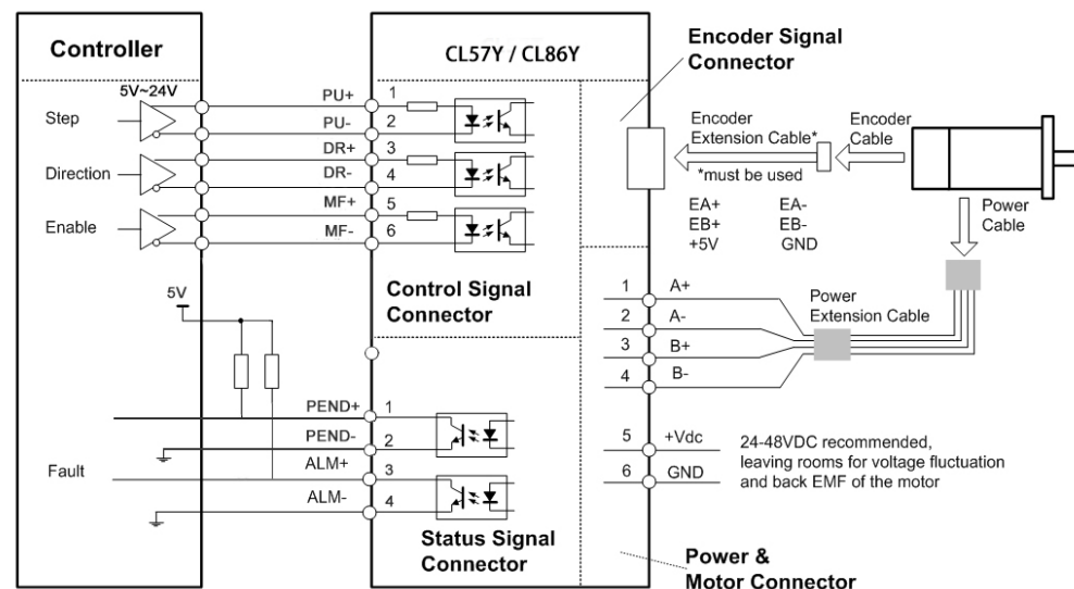
Figure 3: Typical connection
