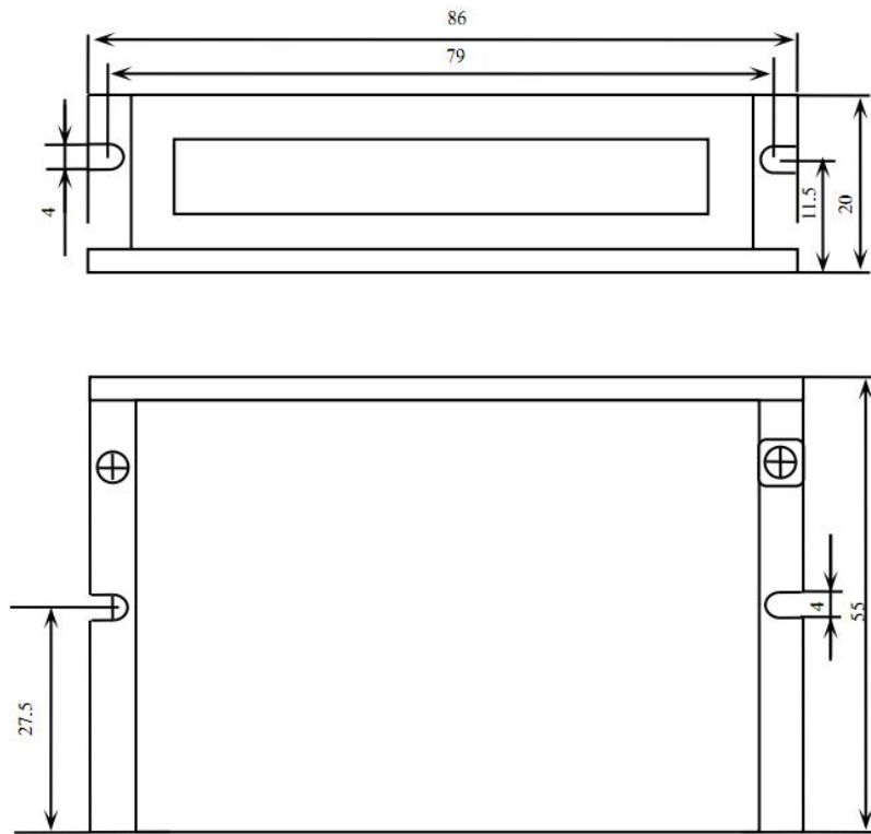
Figure 1: Mechanical specifications
