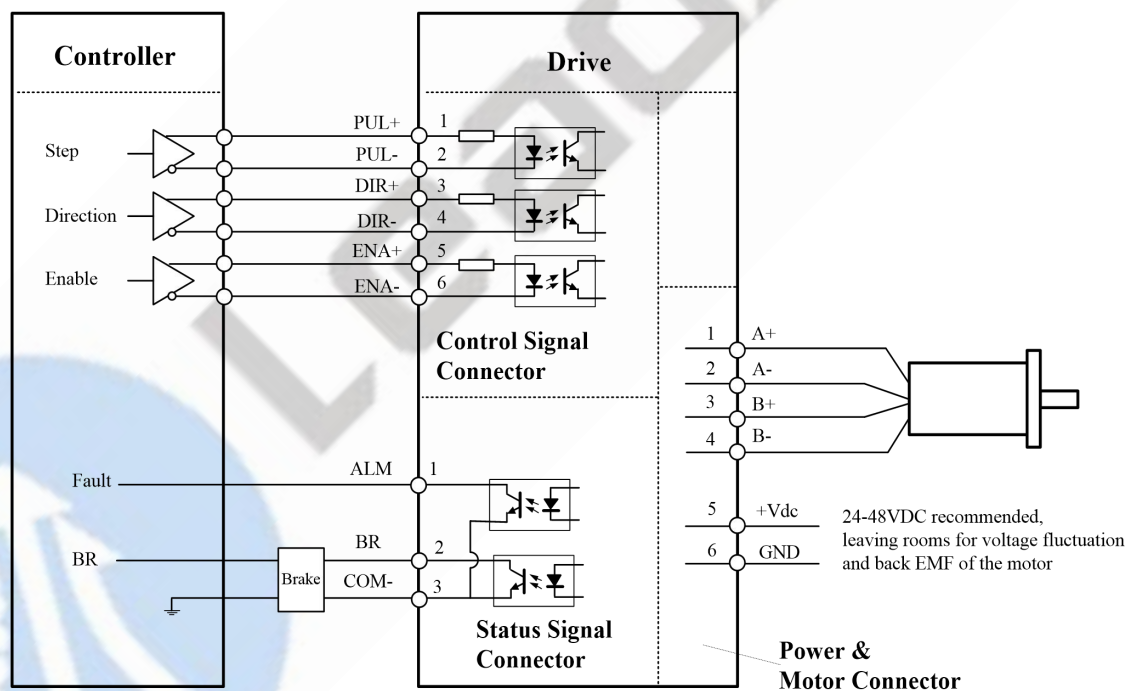
Figure 12 Typical connection
