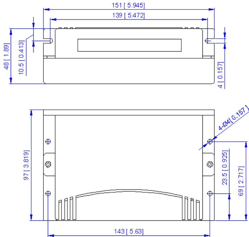
Figure 1: Mechanical specifications
